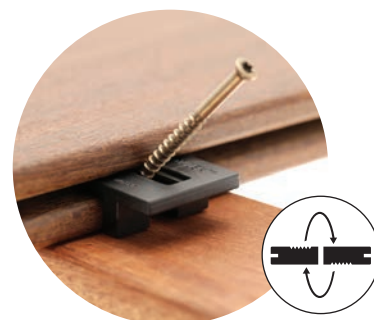
Screwing down of boards into the joists
